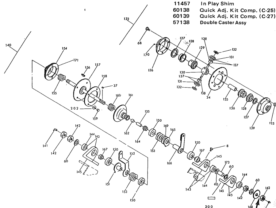
Lock Washer (Not Shown) is PN 11515
